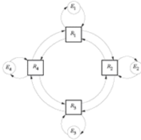
Fig 2.1: The physical topology of a typical WDM network with four end-nodes E1—E4 and four routers R1—R4.(S. Bandyopadhyay, 07. page 4.)
