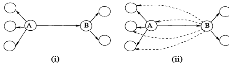
Figure 3: Name Dropper (Harchol-Balter, 1999, page: 235)
