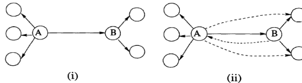
Figure 2: Random Pointer Jump with Back Edge (Harchol-Balter, 1999, page: 233)
