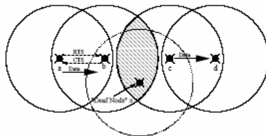
Figure 1: Deaf Node Situation (Ref. [43], Page: 1)
