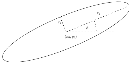
Figure 1: An ellipse
